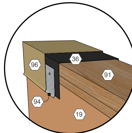
Outside View of Coping Cap
