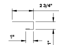
HEAD/JAMB TRIM
