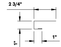
HEAD/JAMB TRIM
