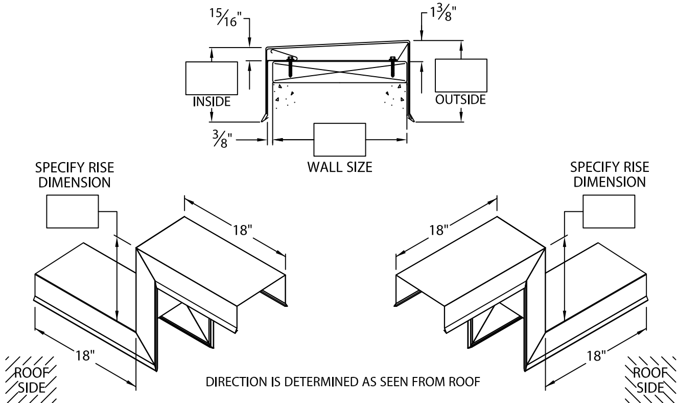
LEFT HAND STEP-UP MITER
